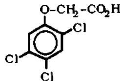
2, 4, 5-T
